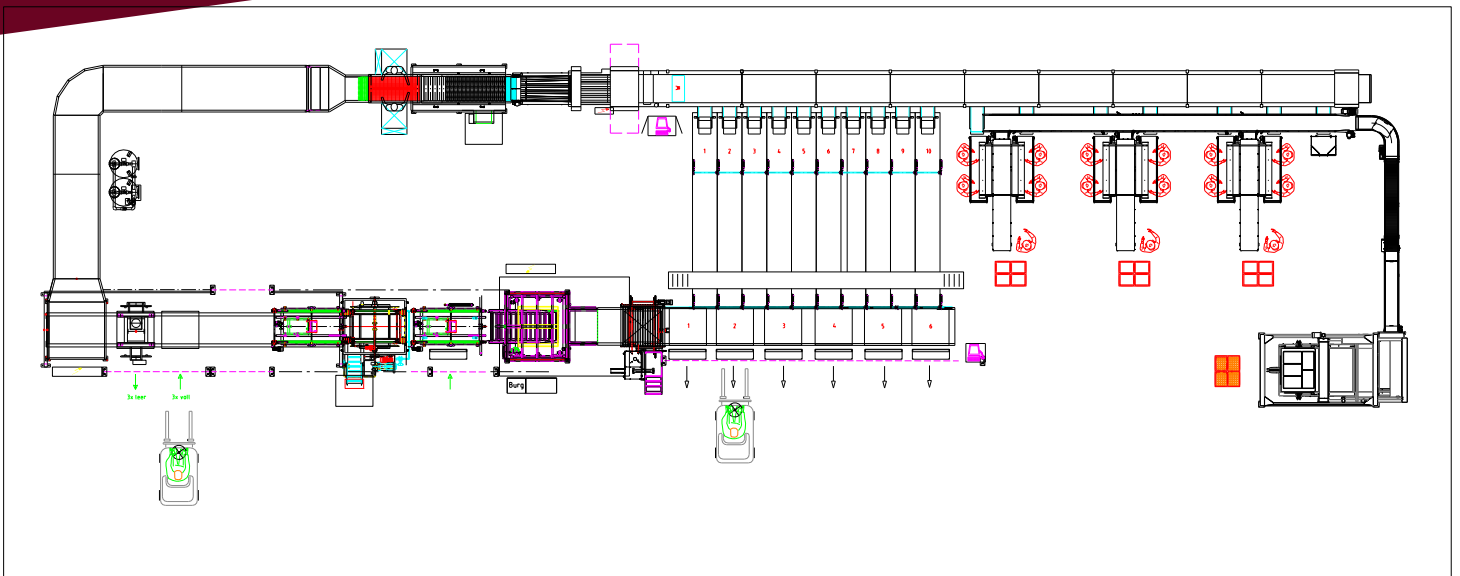
Pre-sorting line for apples with short channels (example)
