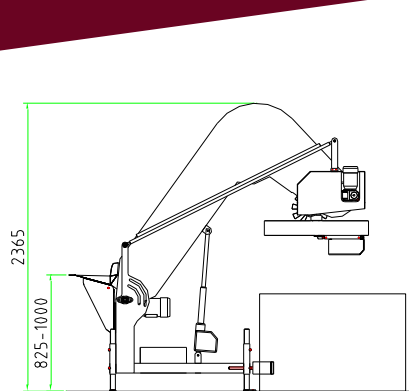
Sideview BGV-series
